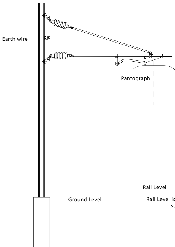
Standard Mk1 25KV OLE mast (pull off registration) Set at working minimal height of 4190mm
