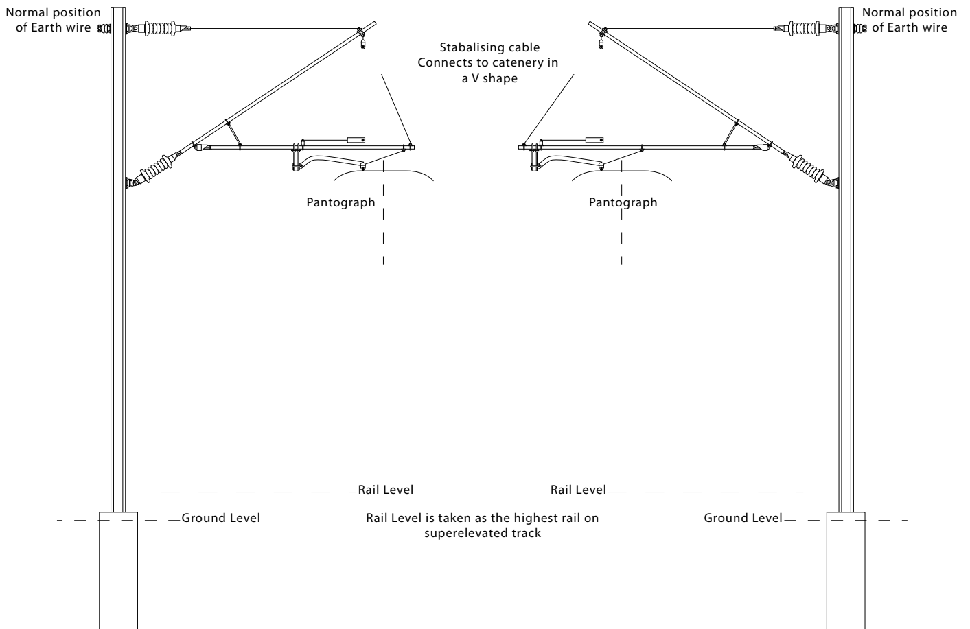
Standard Mk1 25KV OLE mast (pull off registration, compound catenary) Set at normal working height of 4720mm
